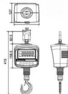
Dimensions(mm)
